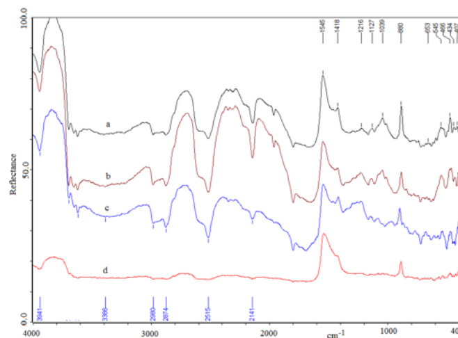
Figure 3: Micro-FTIR spectra of Noravank stone: a) external red point of a stone, b) external red point of the cut Areni stone, c) clear inner point of the cut Noravank stone d) dark inner point of the cut Noravank stone.
