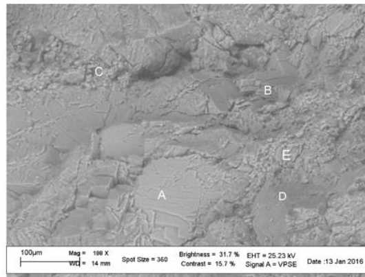
Figure 6: Sample area investigated with analysis EDS in the points indicated by the letters and compositions indicated in Table 1.
