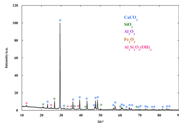
Figure 2: XRD spectra corresponds to Armenian ochre characteristics.
